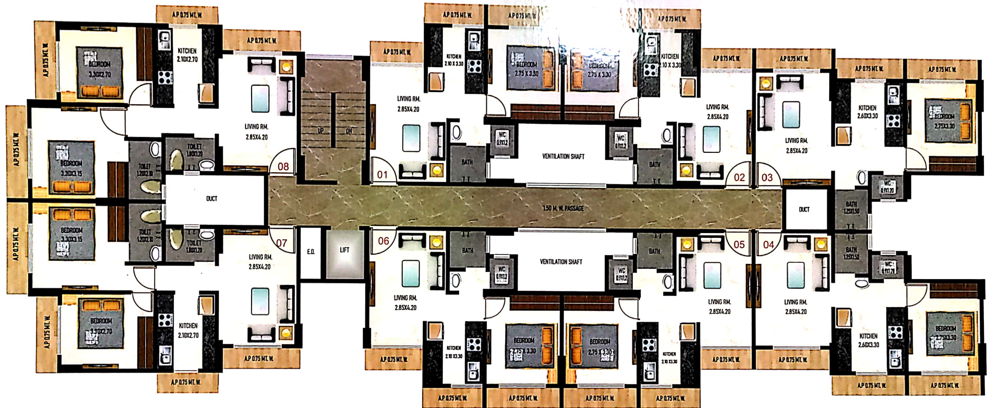
1ST TO 6TH FLOOR PLAN (D-WING)
